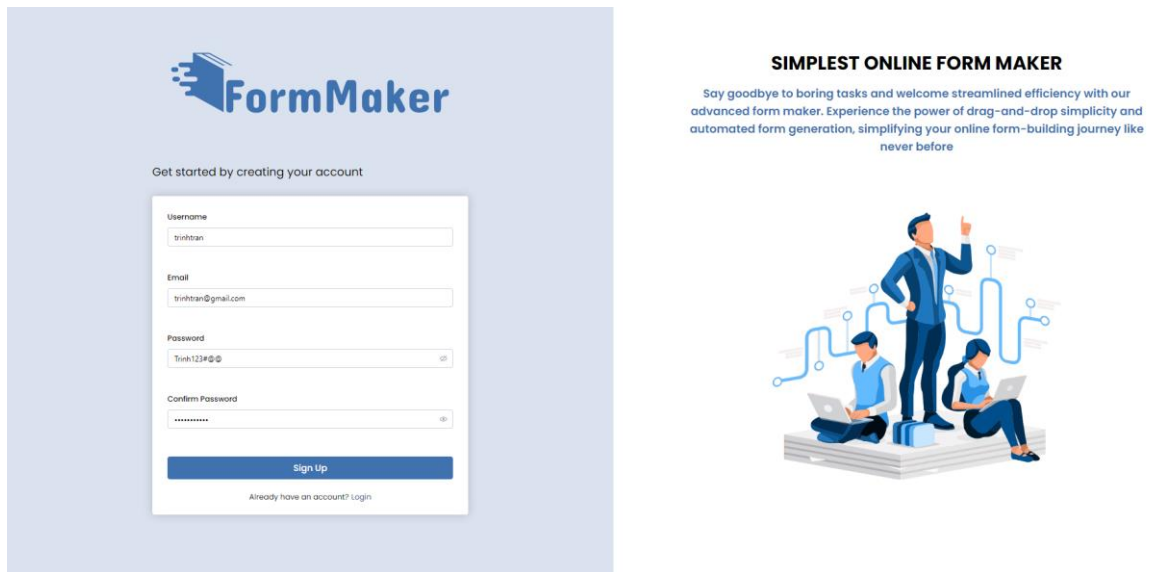
Figure 25. Signup Screen
