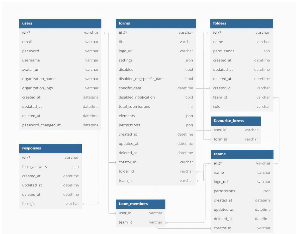
Figure 18. Database design
