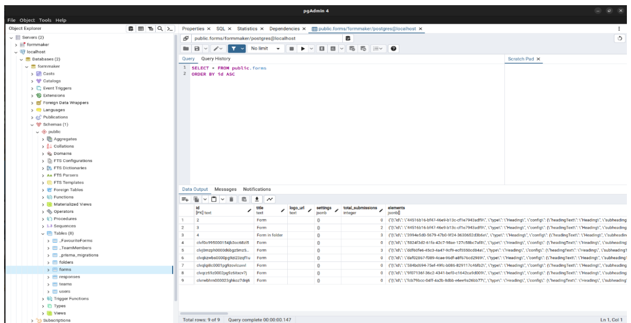
Figure 3. PgAdmin tool
