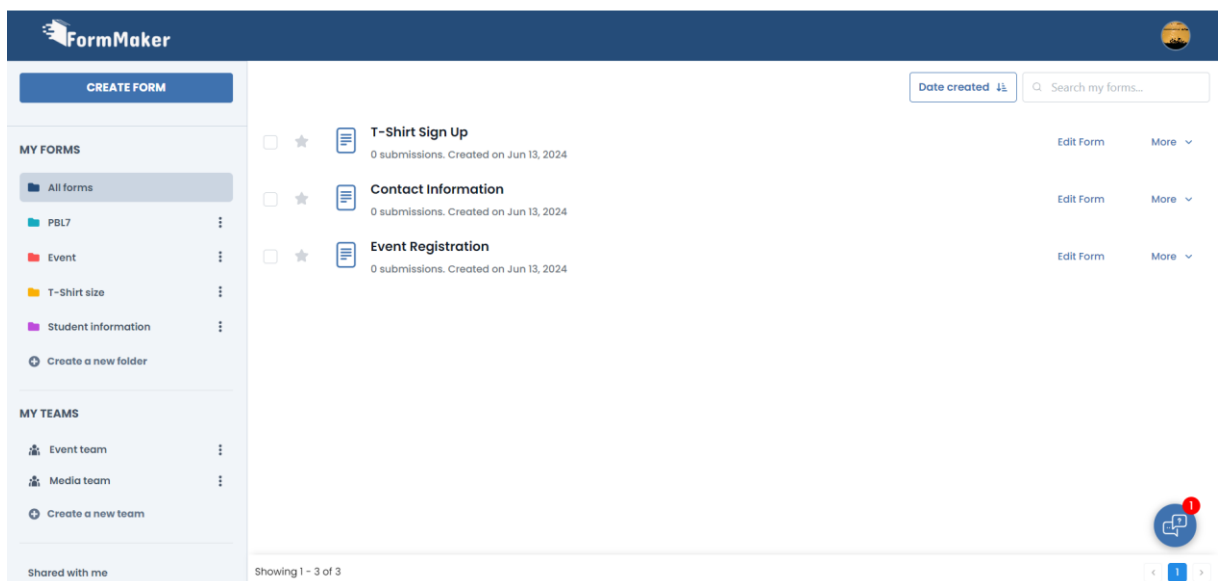
Figure 26. Homepage screen
