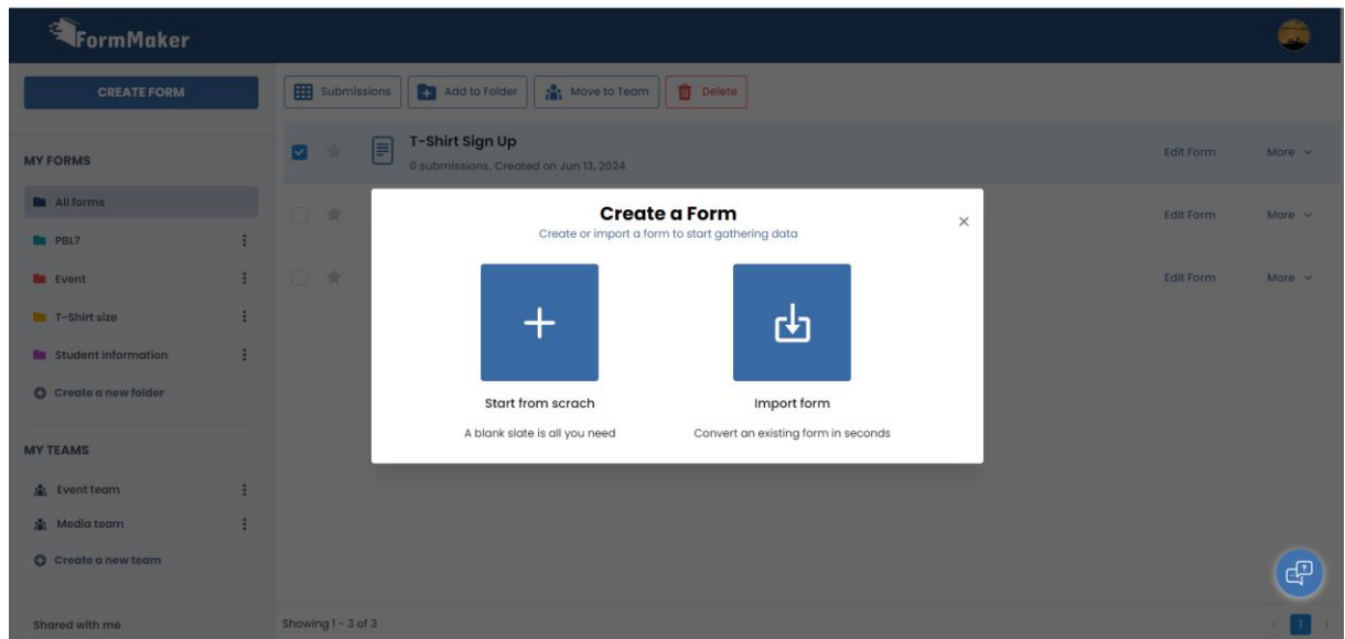
Figure 27. Create form
