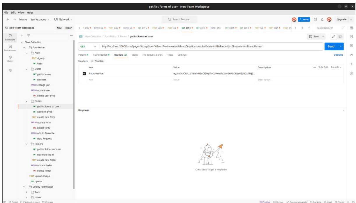
Figure 4. Postman tool
